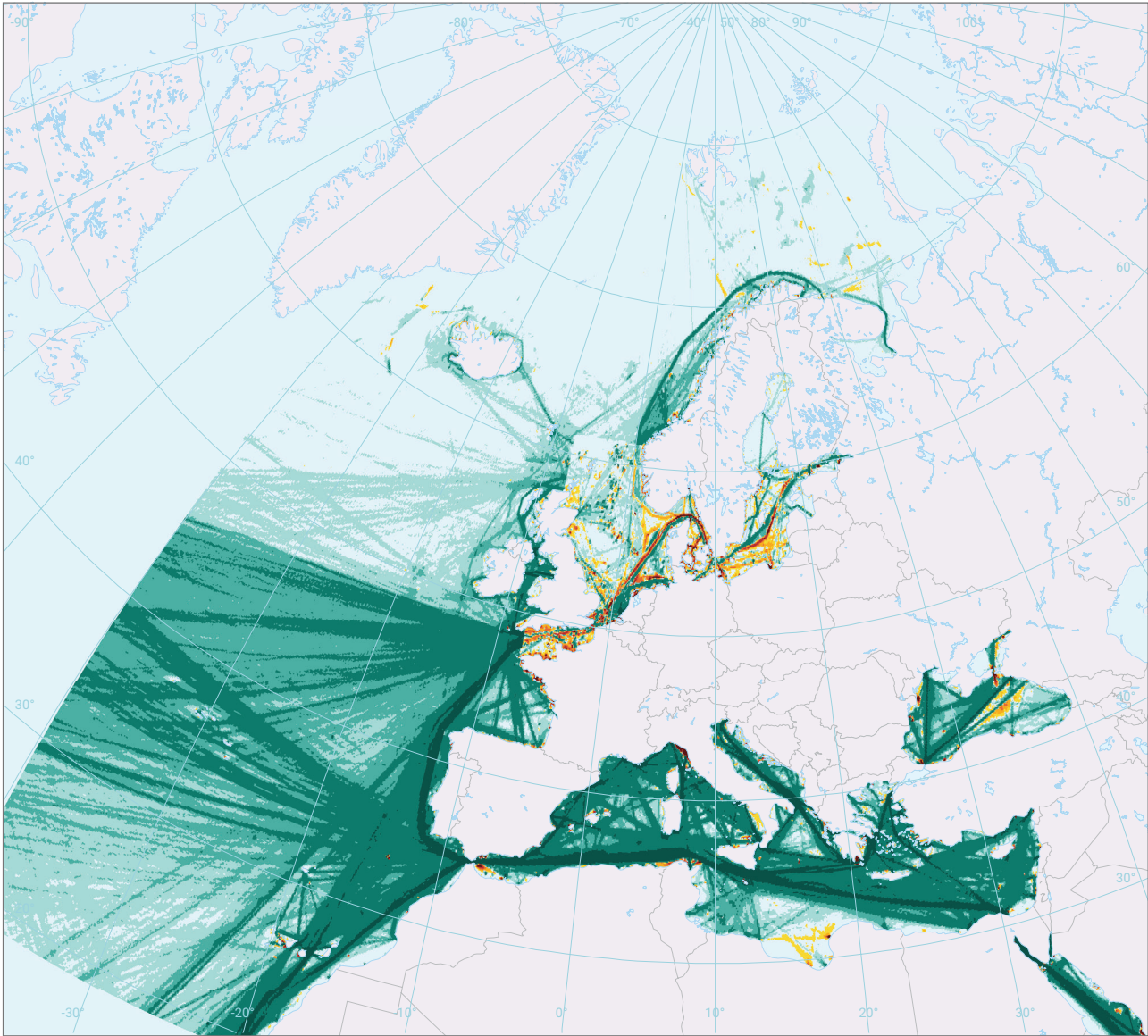
Map 2.6 Difference in PM 2.5 emissions in European shipping areas
